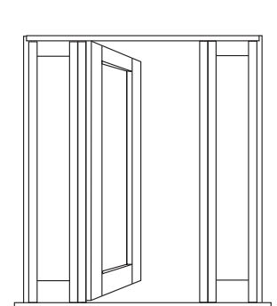
System 4 One Door/ Two Sidelites
