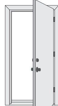
Right-Hand Outswing
